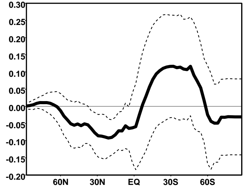
Ocean Heat Transport Years (61-80) Minus Years (1-20)
