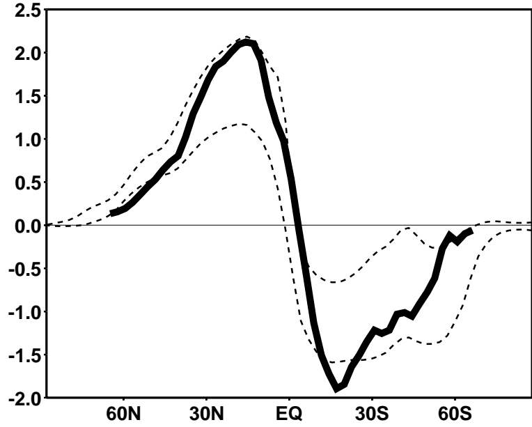
Ocean Heat Transport
