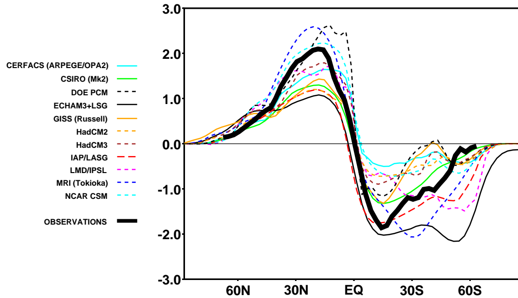
Ocean Heat Transport
