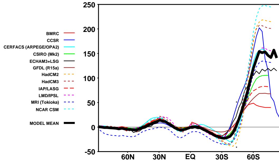
Zonally-Averaged Barotropic Streamfunction
