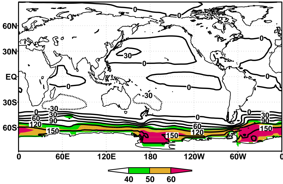
Barotropic Streamfunction Model Mean Contoured Model Standard Deviation Shaded
