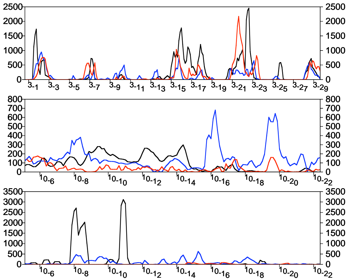
Figure 10. Time series of vertically integrated LWC (gm/m 2 ) at the SGP (top, March 2000), NSA (middle, October 2004) and TWP (bottom, October 2004). Microbase=black, CAM3=blue AM2= red
