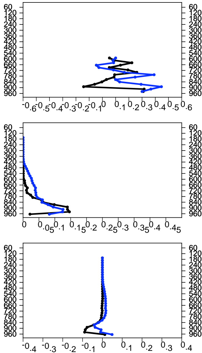
Figure 8. Comparisons of LWC (gm/m3) at the NSA. (CAM3=Blue and AM2=Black). Correlation (top), RMS (middle) Bias (bottom).
