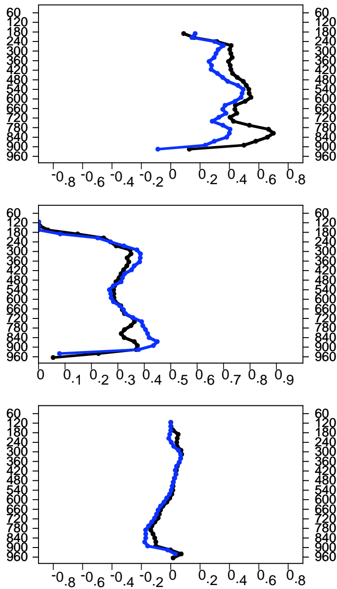
Figure 2. Comparisons of cloud fraction at the SGP. (CAM3=Blue and AM2=Black). Correlation (top), RMS (middle) Bias (bottom).
