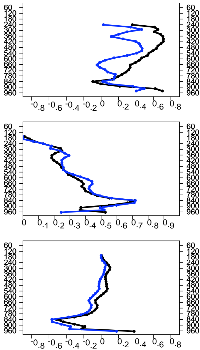
Figure 3. Comparisons of cloud fraction at the NSA. (CAM3=Blue and AM2=Black). Correlation (top), RMS (middle) Bias (bottom).
