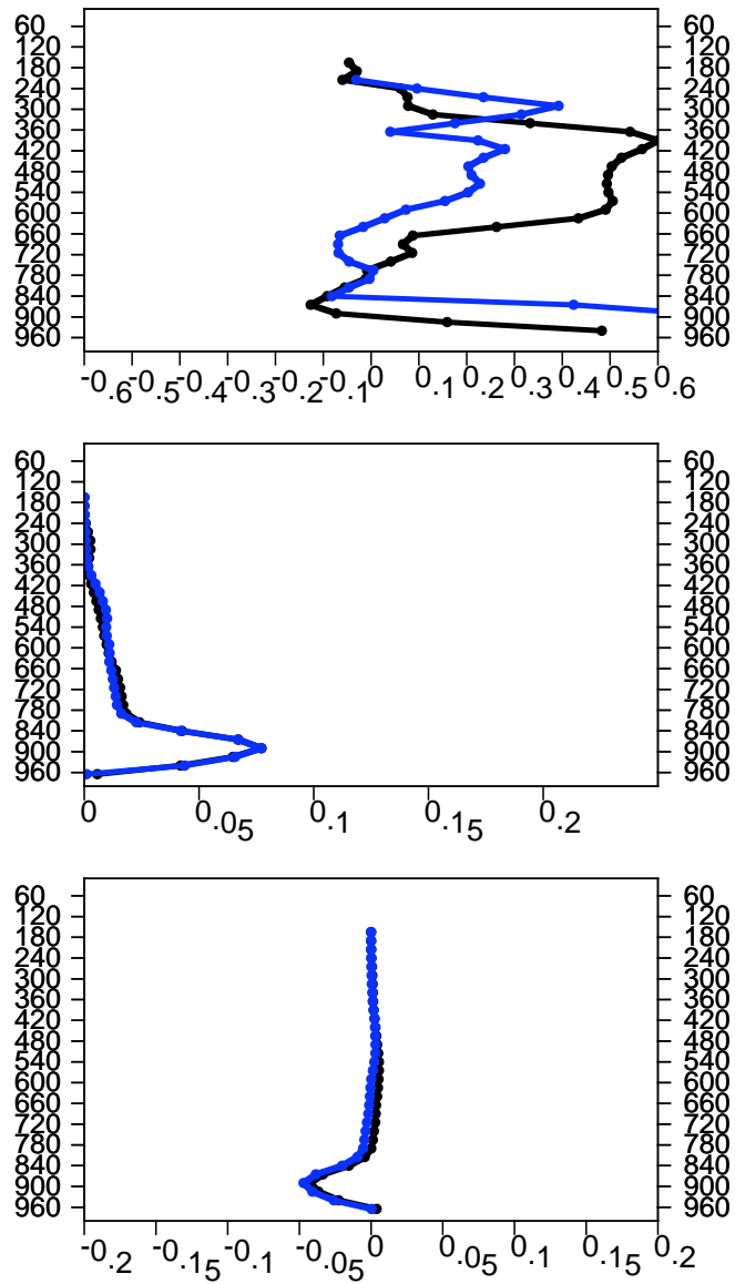
Figure 13. Comparisons of IWC (gm/m3) at the NSA. (CAM3=Blue and AM2=Black). Correlation (top), RMS (middle) Bias (bottom).
