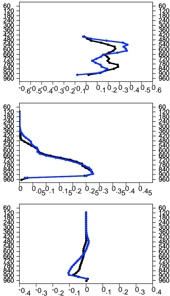
Figure 7. Comparisons of LWC (gm/m3) at the SGP. (CAM3=Blue and AM2=Black). Correlation (top), RMS (middle) Bias (bottom).
