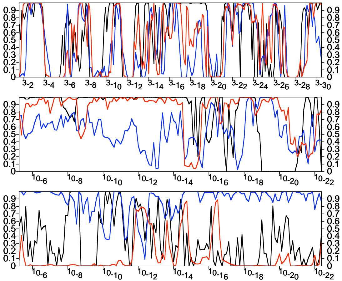
Figure 5. Time series of vertically integrated cloud fraction at the SGP (top, March 2000), NSA (middle, October 2004) and TWP (bottom, October 2004). Microbase=black, CAM3=blue AM2= red
