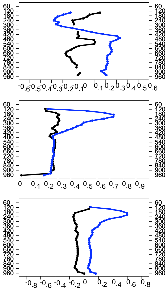
Figure 4. Comparisons of cloud fraction at the TWP. (CAM3=Blue and AM2=Black). Correlation (top), RMS (middle) Bias (bottom).
