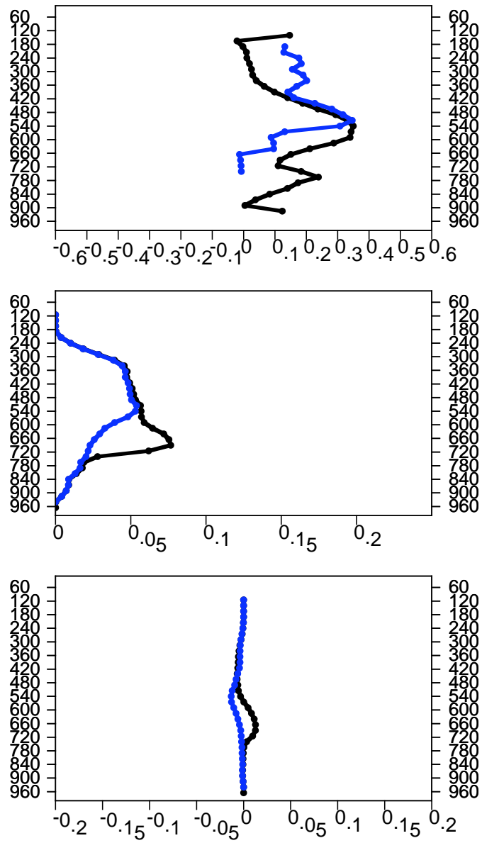
Figure 12. Comparisons of IWC (gm/m 3 ) at the SGP. (CAM3=Blue and AM2=Black). Correlation (top), RMS (middle) Bias (bottom).
