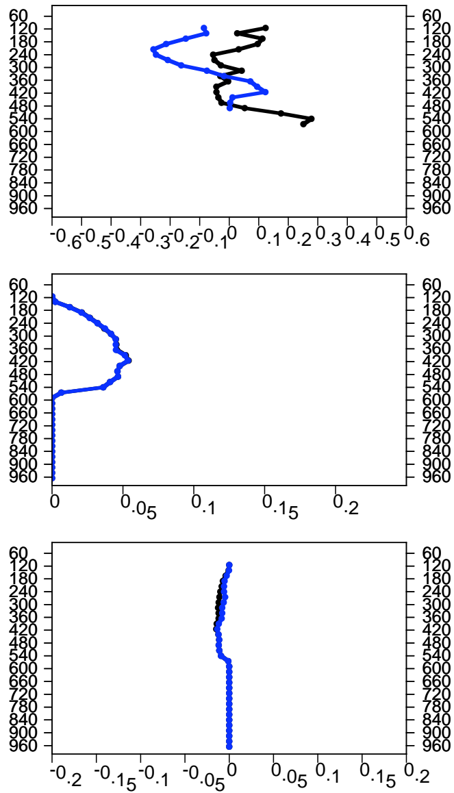
Figure 14. Comparisons of IWC (gm/m 3 ) at the TWP. (CAM3=Blue and AM2=Black). Correlation (top), RMS (middle) Bias (bottom).
