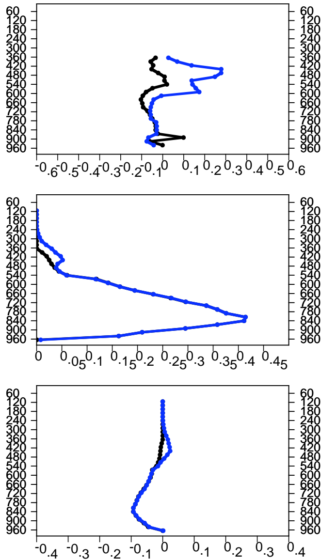
Figure 9. Comparisons of LWC (gm/m 3 ) at the TWP. (CAM3=Blue and AM2=Black). Correlation (top), RMS (middle) Bias (bottom).
